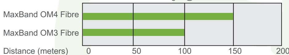
10Gb/s Link Length @850nm Based on IEEE802.3ae
