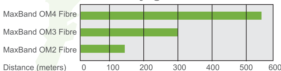
10Gb/s Link Length @850nm Based on IEEE802.3ae
